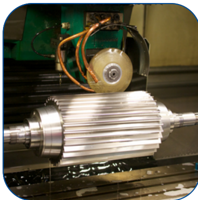
Sharpening Milling Cutter
